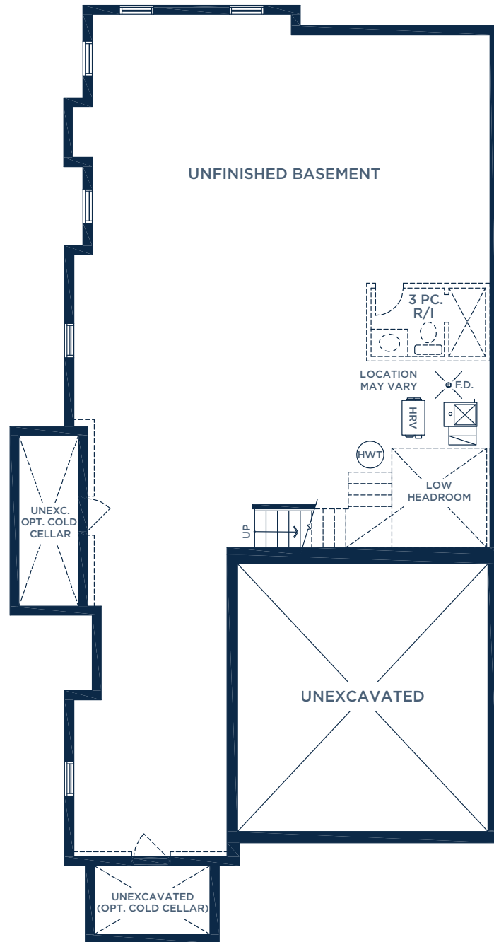
LOWER LEVEL PLAN ELEV. B
