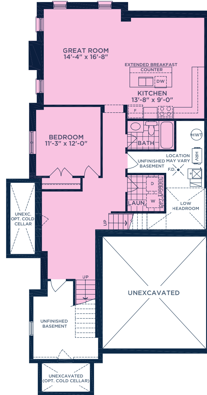
OPT. FLEXHOUS™ LOWER LEVEL PLAN ELEV. B
