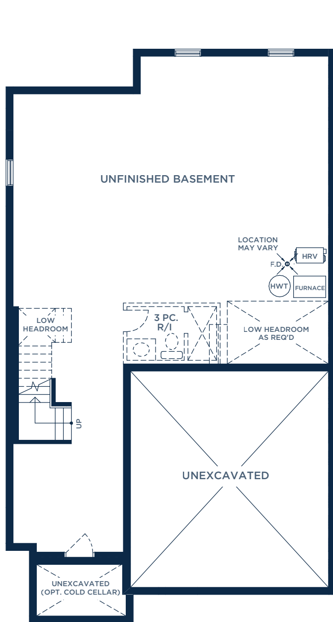
LOWER LEVEL PLAN ELEV. C
