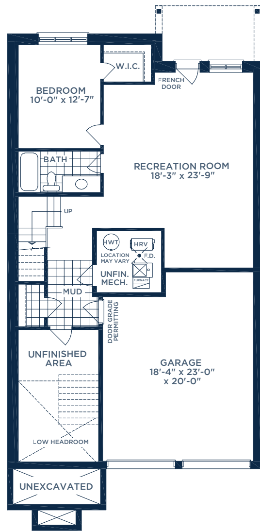
OPT. GROUND FLOOR PLAN ELEV. C
