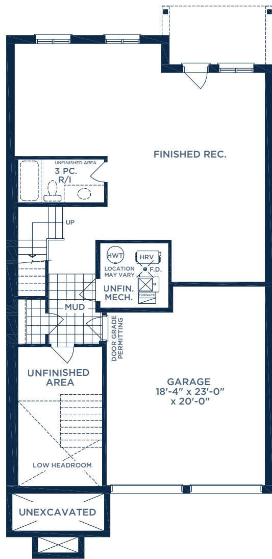
GROUND FLOOR PLAN ELEV. C
