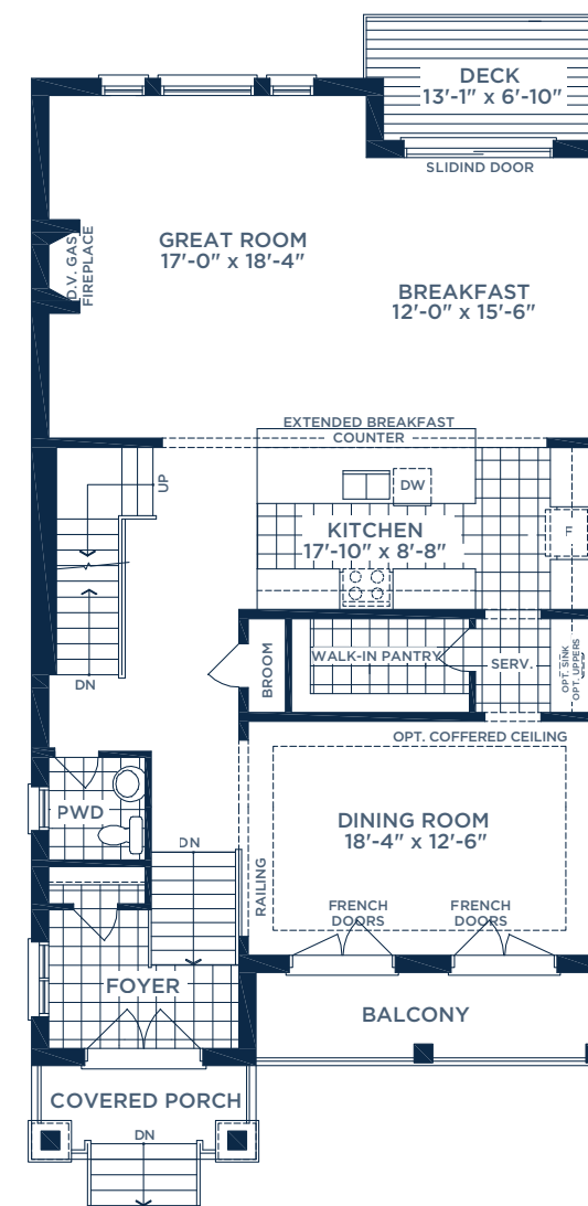
MAIN FLOOR PLAN ELEV. C
