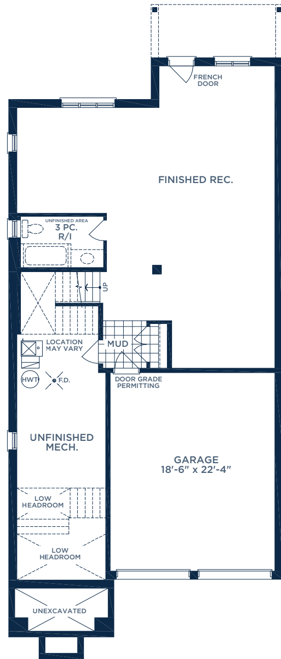
GROUND FLOOR PLAN ELEV. B
