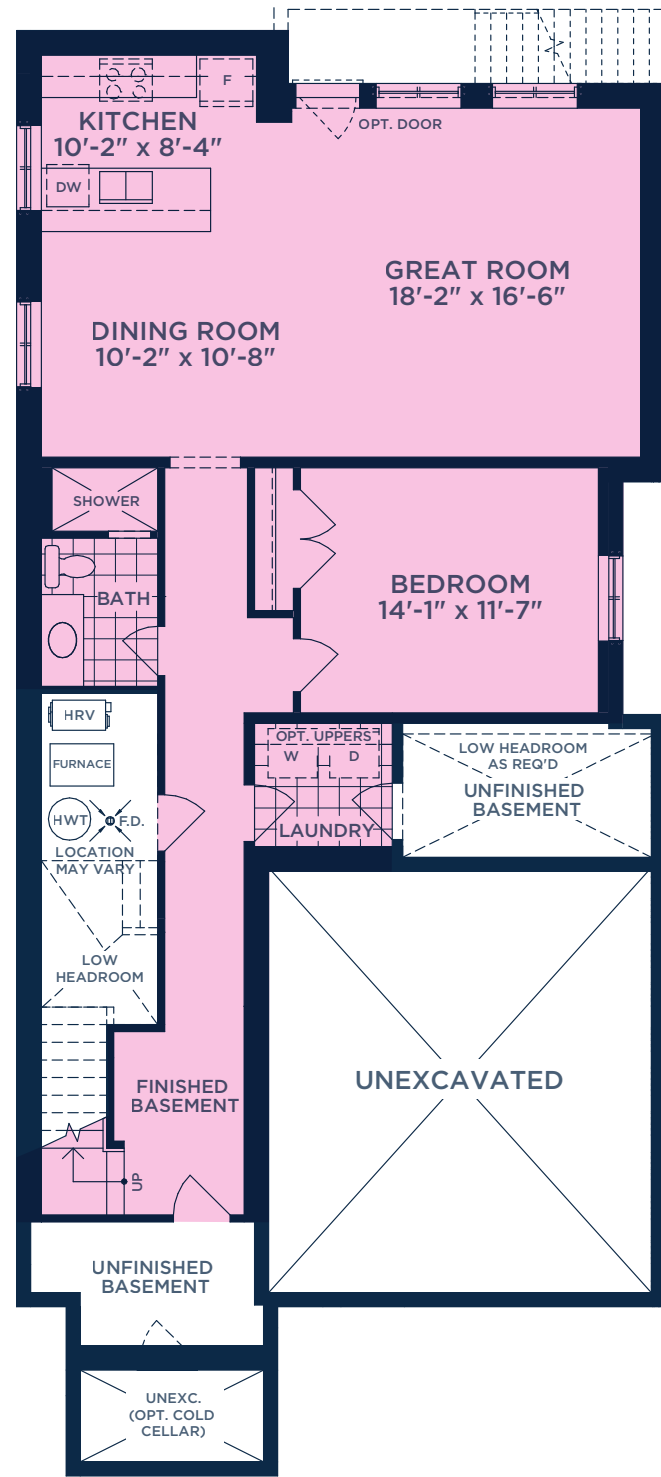
OPT. FLEXHOUS™ LOWER LEVEL PLAN ELEV. A (B & C SIMILAR)
