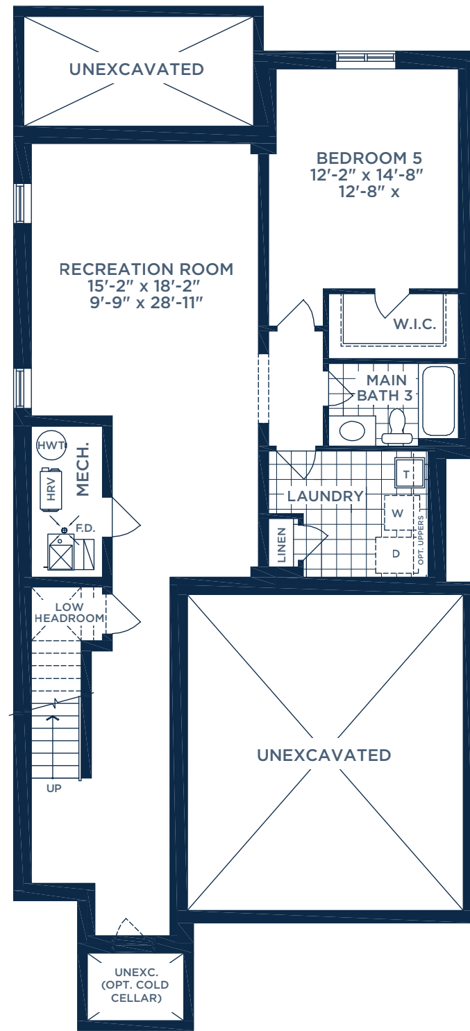
OPT. LOWER LEVEL PLAN ELEV. B
