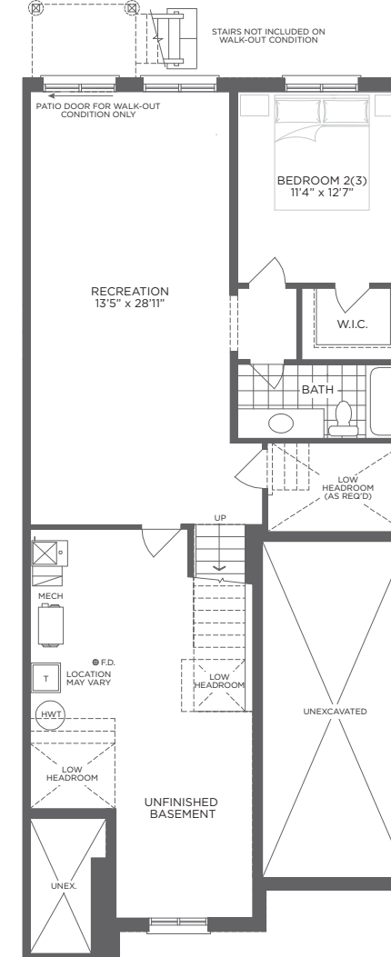
OPTIONAL LOWER LEVEL ELEVATION B FINISHED WITH REC ROOM & 1 BEDROOM
