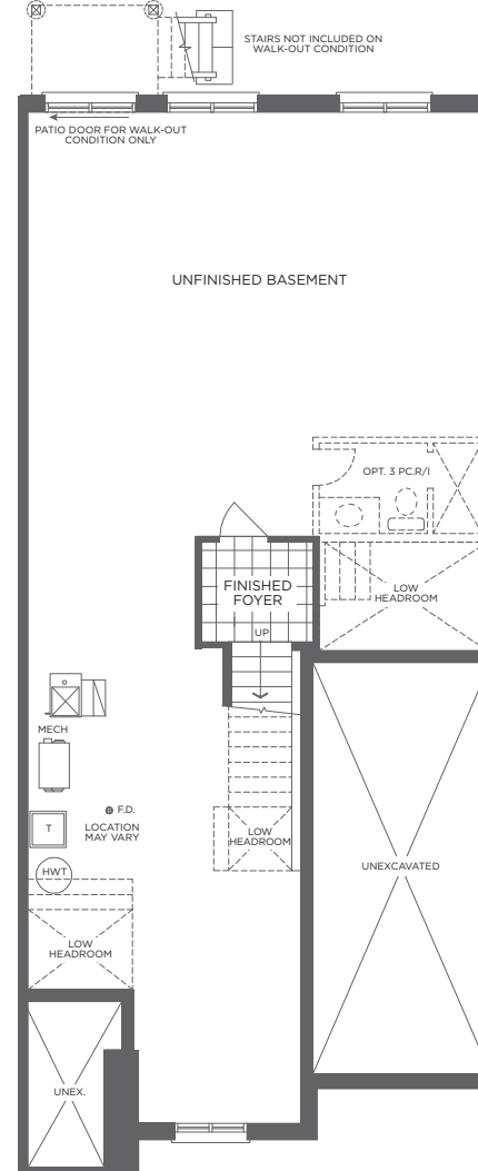
STANDARD LOWER LEVEL ELEVATION B FINISHED FOYER
