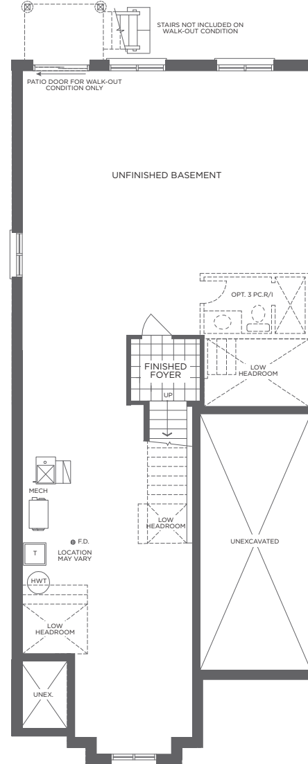
STANDARD LOWER LEVEL ELEVATION C FINISHED FOYER
