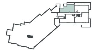
LEVEL 5
