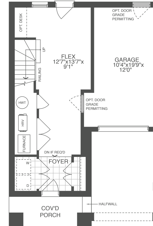
GROUND FLOOR PLAN (A1 & A2)
