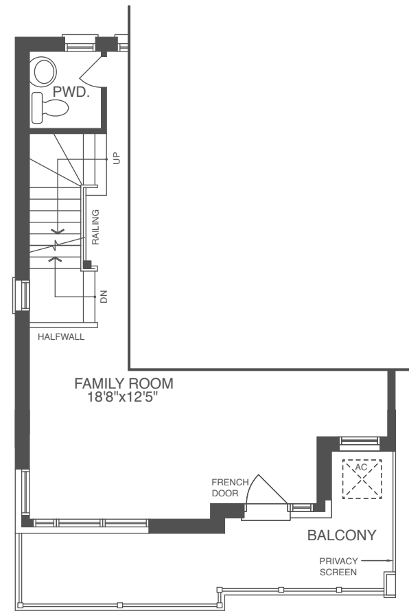
MAIN FLOOR PLAN (A3)
