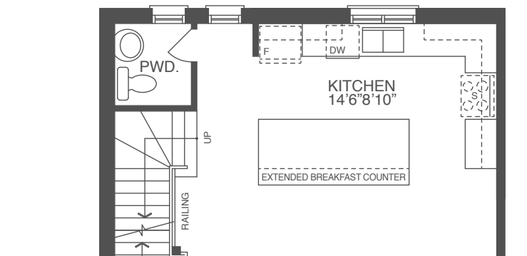
ALTERNATE KITCHEN FLOOR PLAN (A1 & A2)
