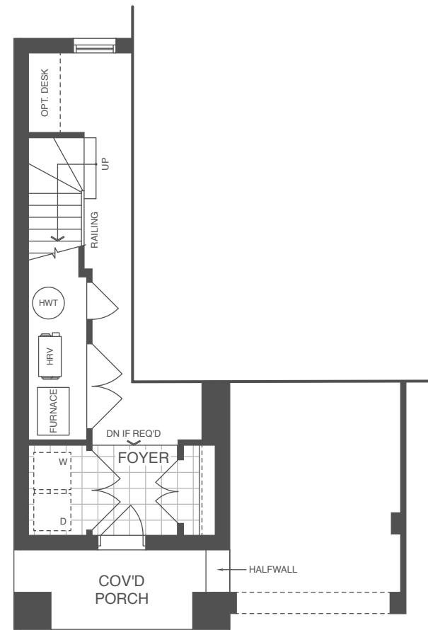
GROUND FLOOR PLAN (A3)
