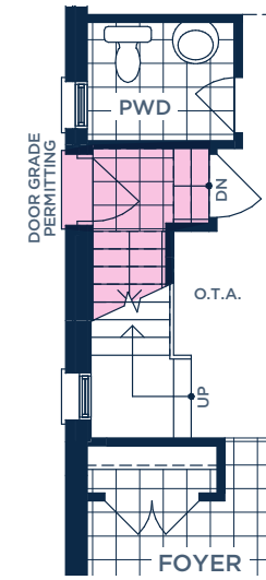
PART. OPT. GROUND FLOOR PLAN FOR OPT. FLEXHOUS™ LOWER LEVEL W/ SIDE DOOR ELEV. A (B & C SIMILAR)
