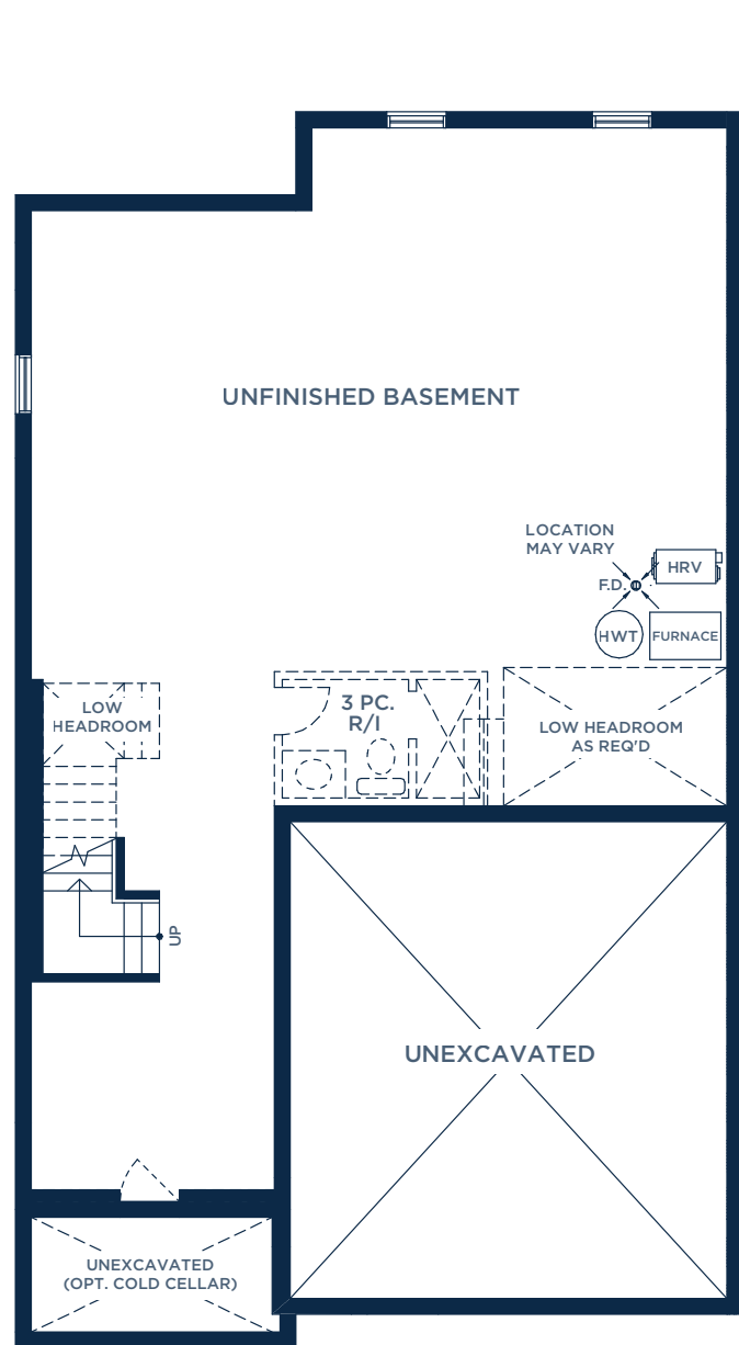
LOWER LEVEL PLAN ELEV. B
