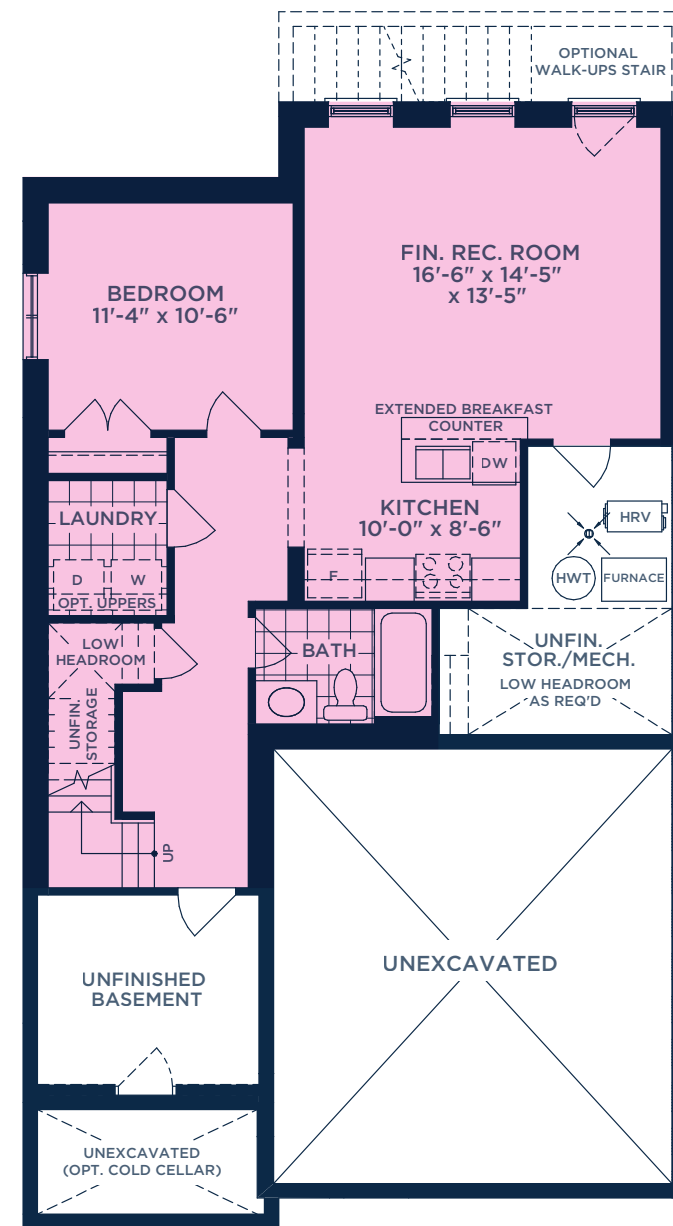
OPT. FLEXHOUS™ LOWER LEVEL PLAN ELEV. B (FOR SIDE DOOR)
