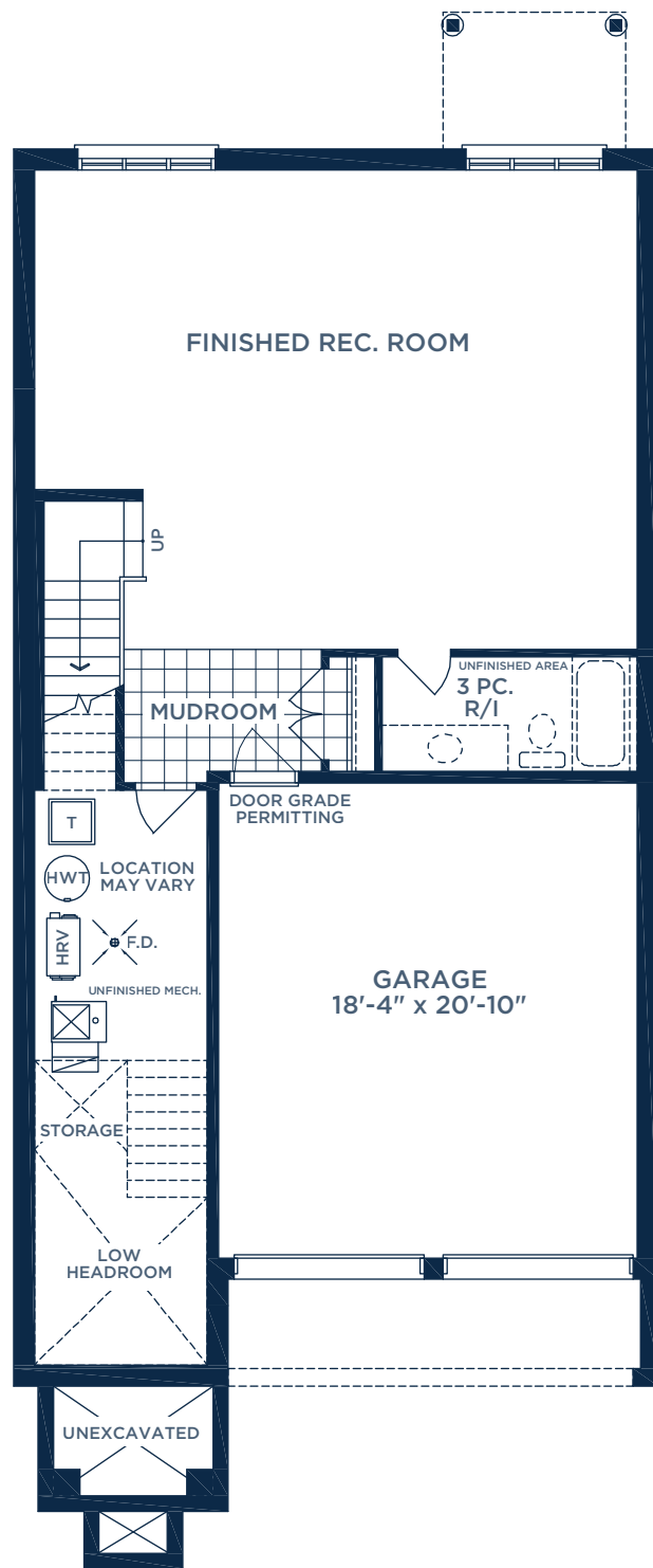
GROUND FLOOR PLAN ELEV. C
