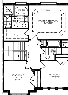
SECOND FLOOR ELEVATION A
