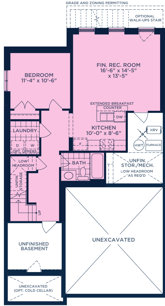
OPT. FLEXHOUZ™ LOWER LEVEL PLAN ELEV. A (FOR SIDE DOOR)
