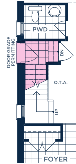
PART. OPT. GROUND FLOOR PLAN FOR OPT. FLEXHOUZ™ LOWER LEVEL W/ SIDE DOOR ELEV. A
