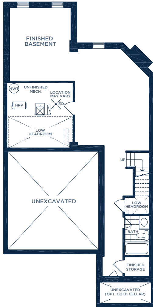
LOWER LEVEL PLAN
