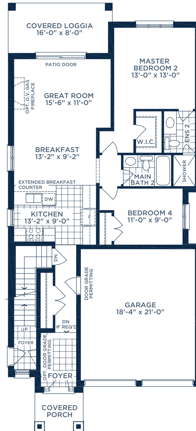
GROUND FLOOR PLAN ELEV. C
