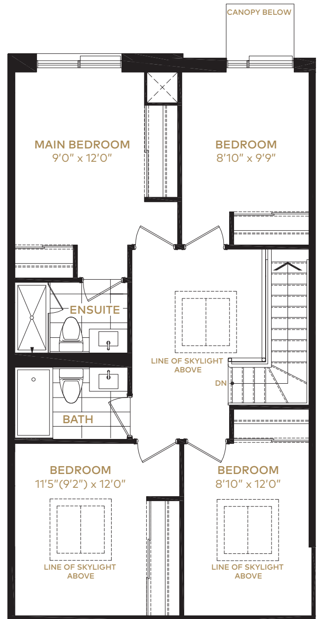
SECOND FLOOR
