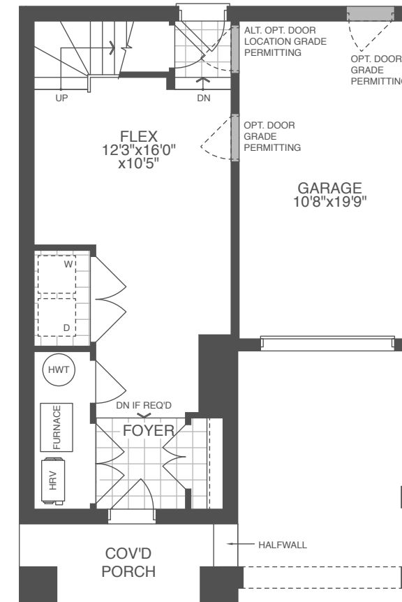
GROUND FLOOR PLAN (A1 & A2)
