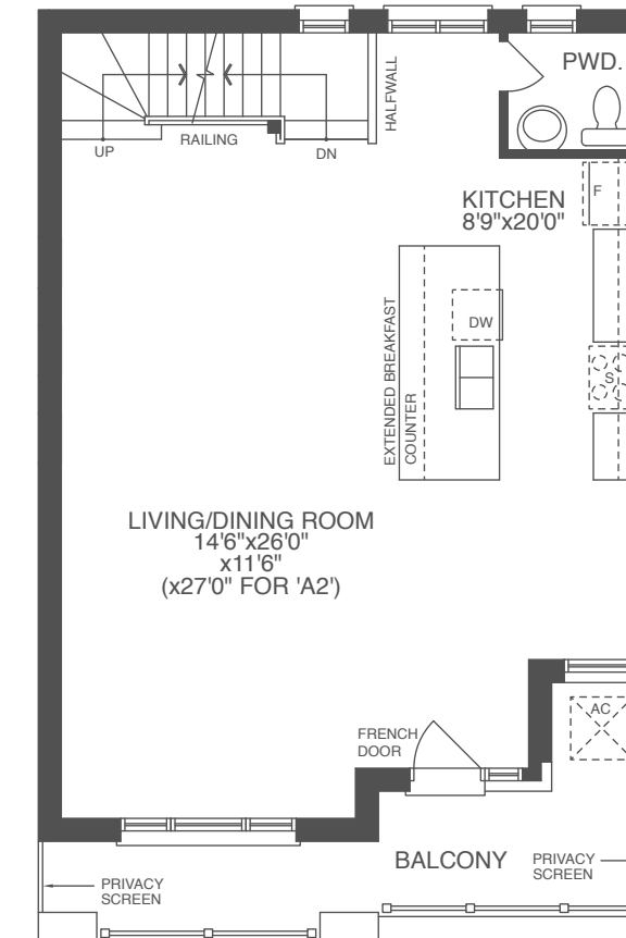
MAIN FLOOR PLAN (A1 & A2)
