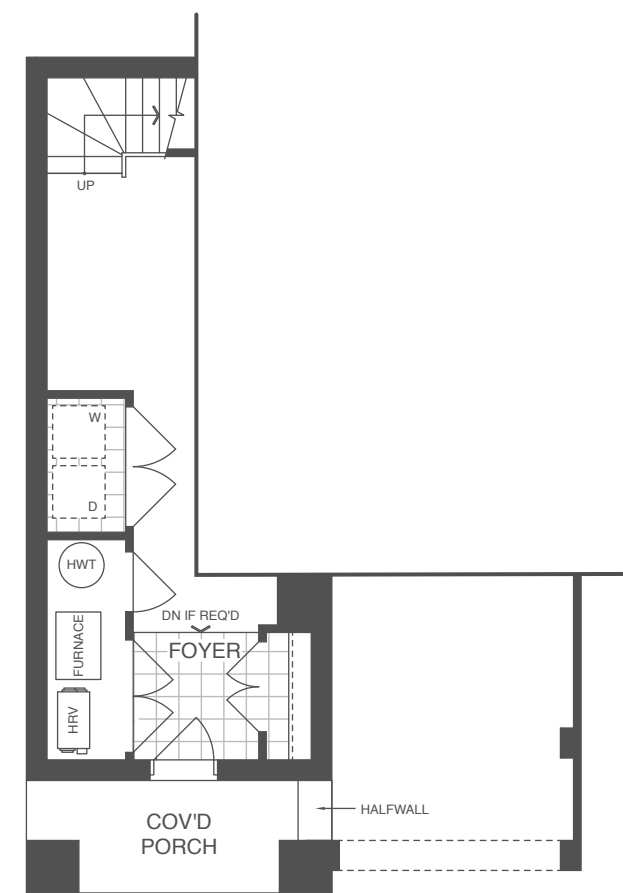
GROUND FLOOR PLAN (A3)
