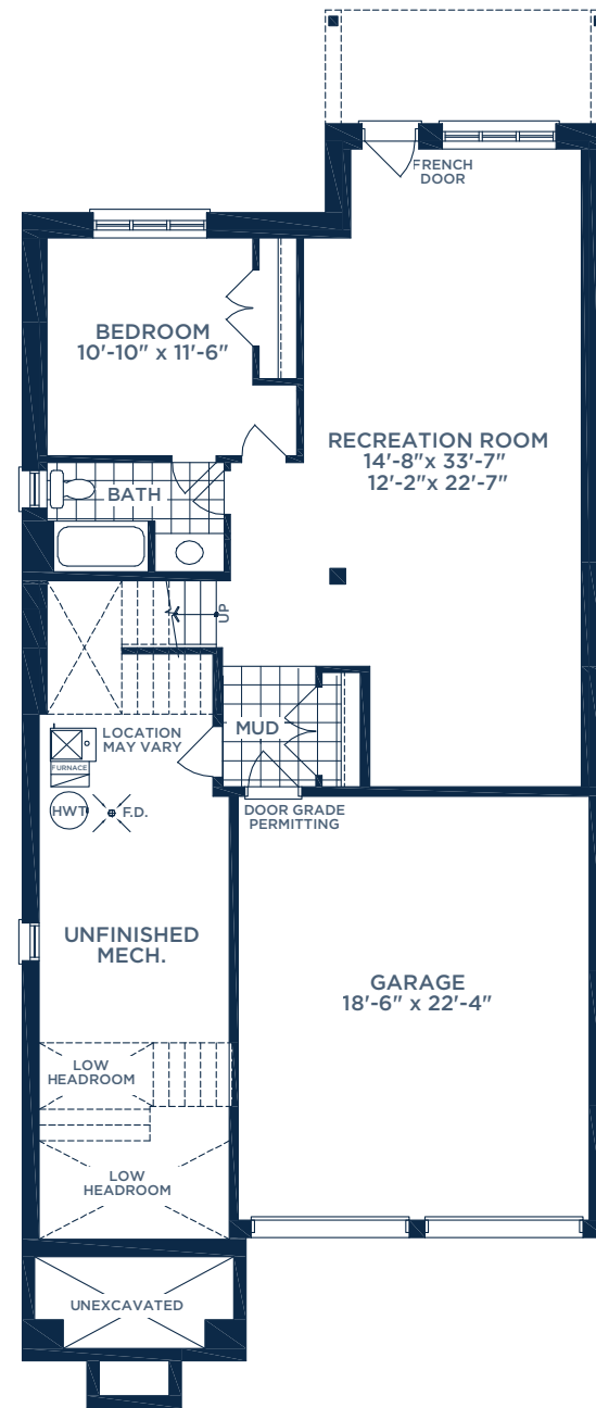
OPT. GROUND FLOOR PLAN ELEV. C
