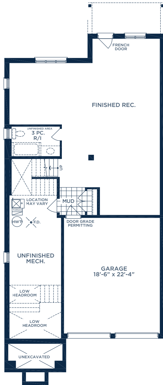
GROUND FLOOR PLAN ELEV. C
