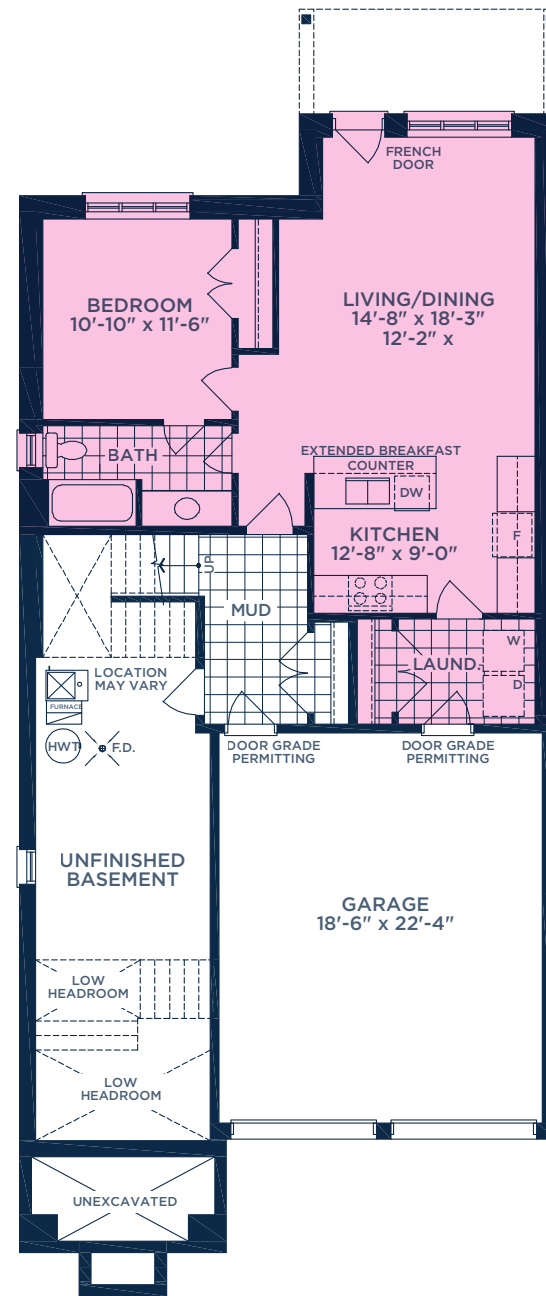
OPT. FLEXHOUS™ GROUND FLOOR PLAN ELEV. C
