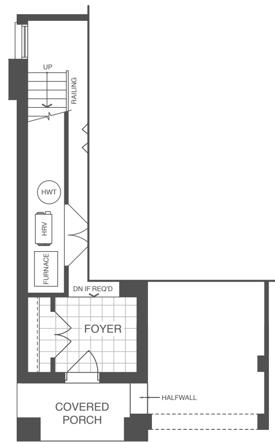
GROUND FLOOR PLAN (A3)
