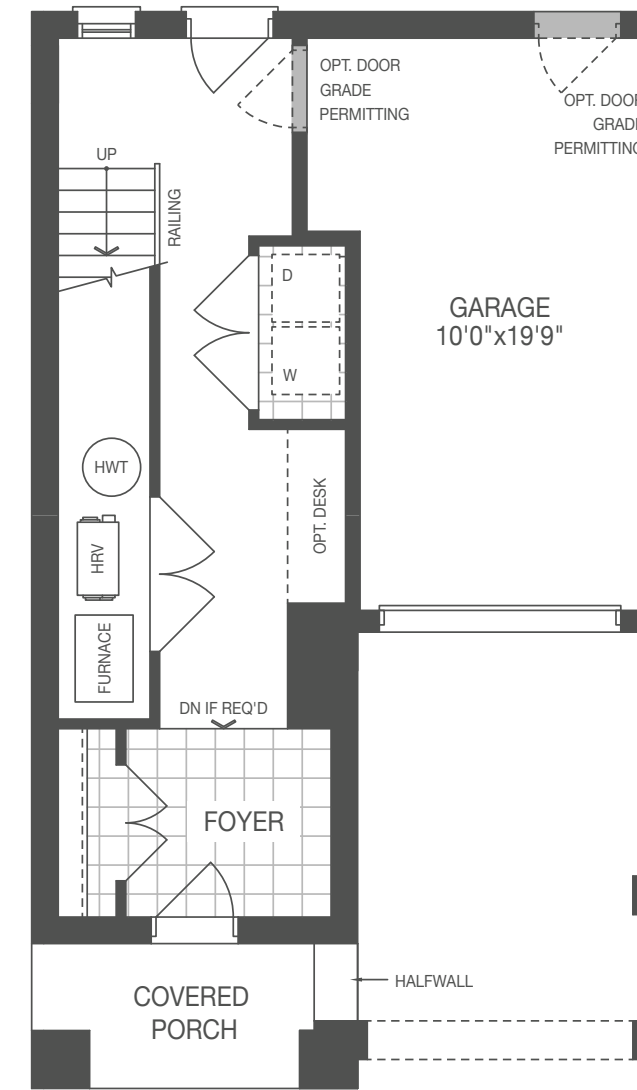
GROUND FLOOR PLAN (A1 & A2)
