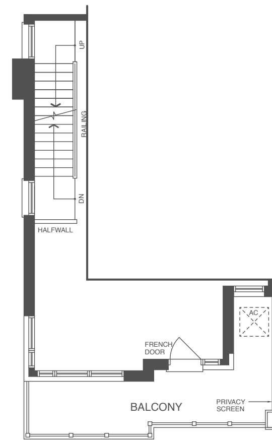
MAIN FLOOR PLAN (A3)
