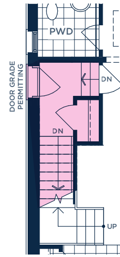
PART. GROUND FLOOR PLAN FOR OPT. FLEXHOUS™ LOWER LEVEL W/ SIDE DOOR ELEV. A
