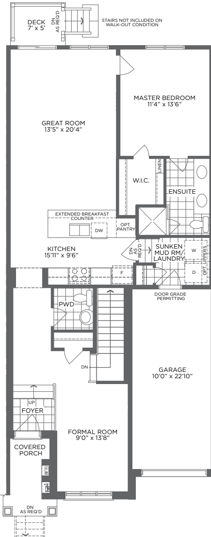
STANDARD MAIN FLOOR ELEVATION A 1 BEDROOM + FORMAL ROOM
