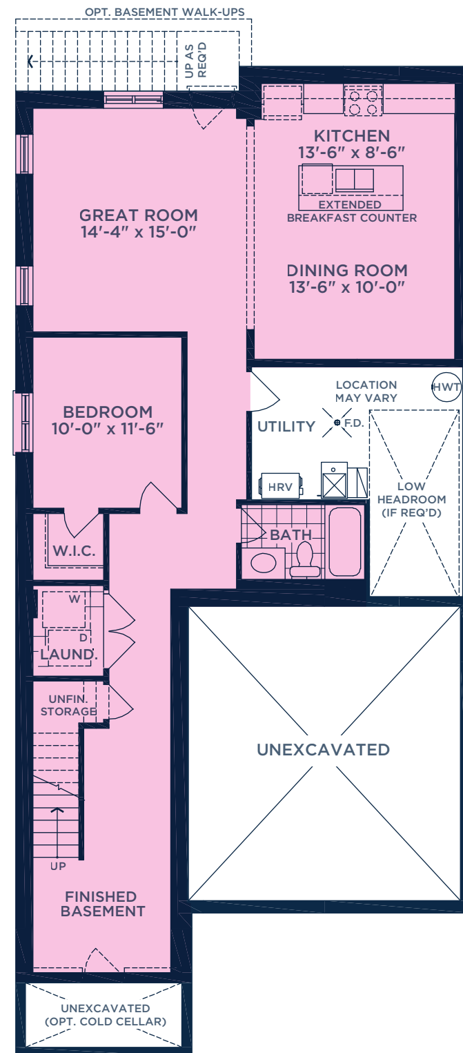
OPT. FLEXHOUS™ LOWER LEVEL PLAN ELEV. C
